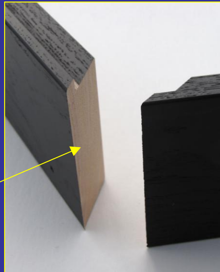
Moulding mitred before underpinning
